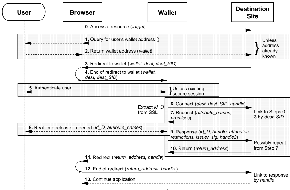
Figure 2 BBAE protocol with parameters. Steps with dashed lines are only needed in certain cases. Secure sessions are required at least for Steps 5, 8, 11, Steps 6, 7, 9, 10, and for Step 12.
