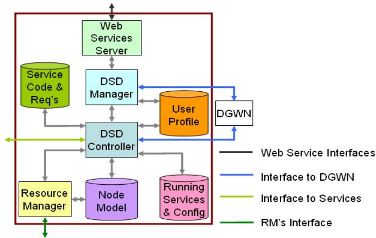
Fig. 2. DSD Architecture
