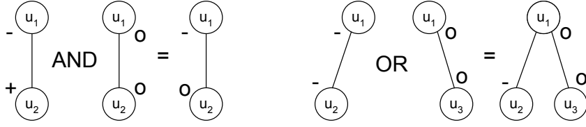
Fig. 1. Examples that EPAL is not closed under conjunction or disjunction.
